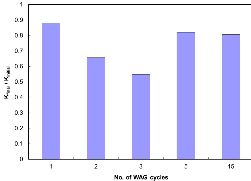
Fig. 6.13—Change in core permeability vs. the change in WAG cycle volume.
