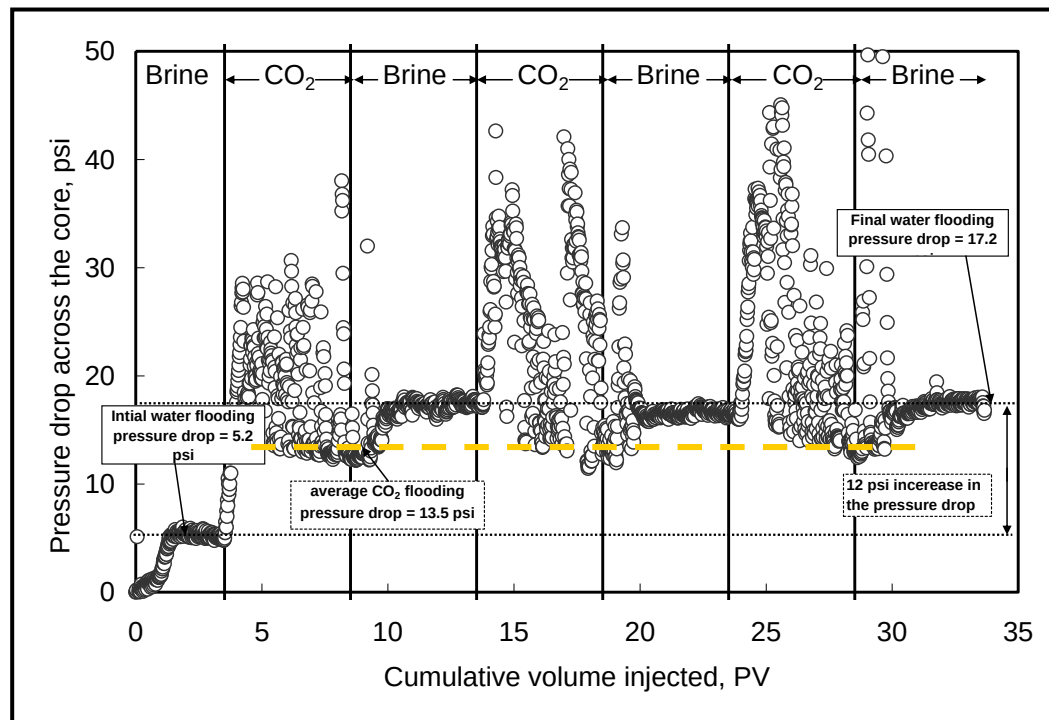
Fig. 6.2— Pressure drop across the core #1, T =200°F, injection flow rate = 5 cm 3 /min
