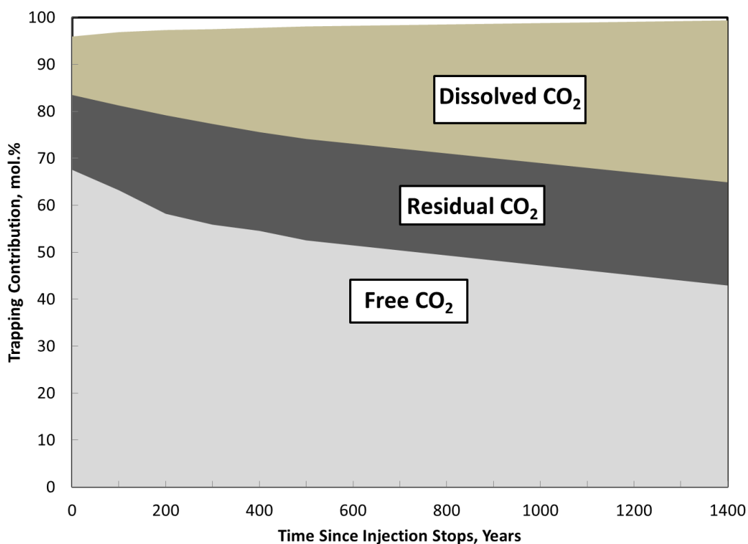
Fig. 5.16— Trapped phases after WAG injection of CO 2 and seawater without sulfate into saline carbonate aquifer
