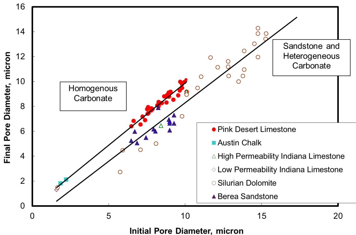
Fig. 8.19—Correlation between initial and final average pore diameter for homogenous and heterogeneous carbonate, and sandstone cores.
