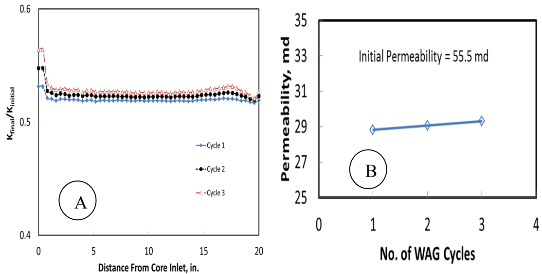
Fig 7.21—Change in core permeability after WAG injection of CO 2 into 20 in. core after injection of 3 WAG cycle of CO 2 : A) permeability distribution across the core, B) overall permeability of the core after each WAG cycle
