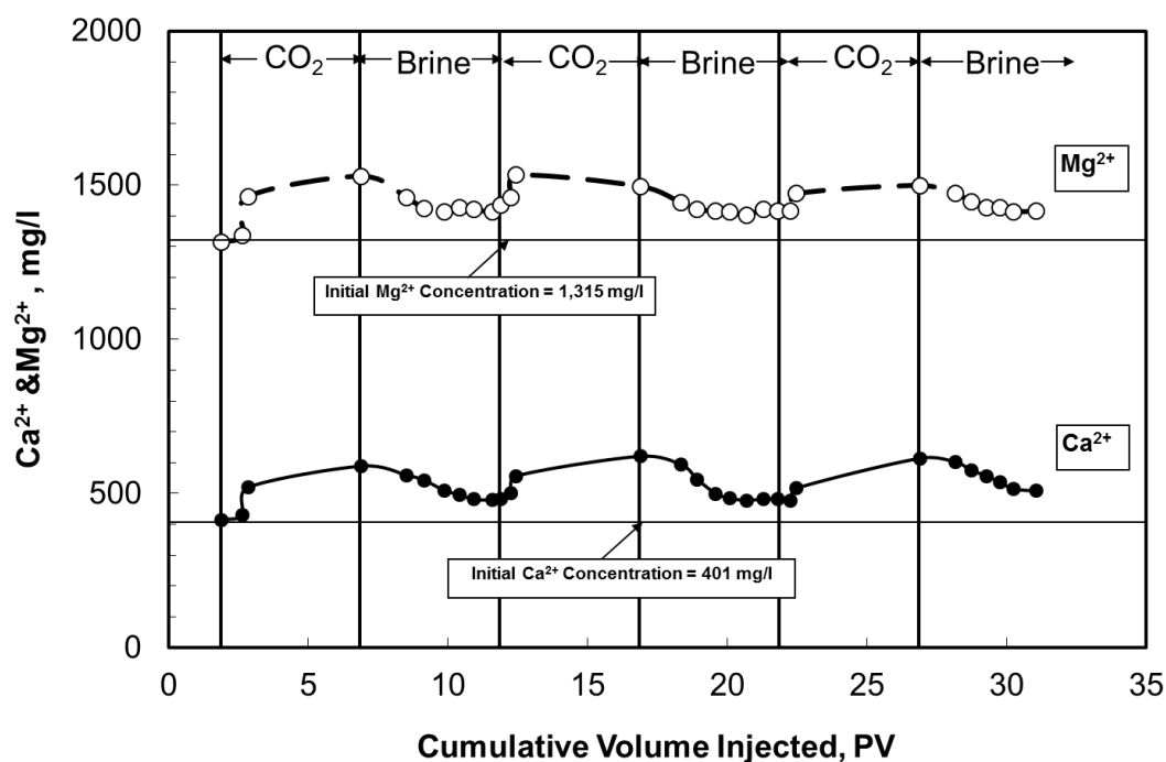
Fig. 7.4—Concentrations of \text{Ca}^{++} and \text{Mg}^{++} in the core effluent samples, core #1
