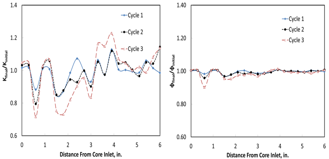
Fig. 5.10—Permeability and porosity distribution at the end of each WAG cycle when WAG injection of CO 2 and seawater conducted for core #5
