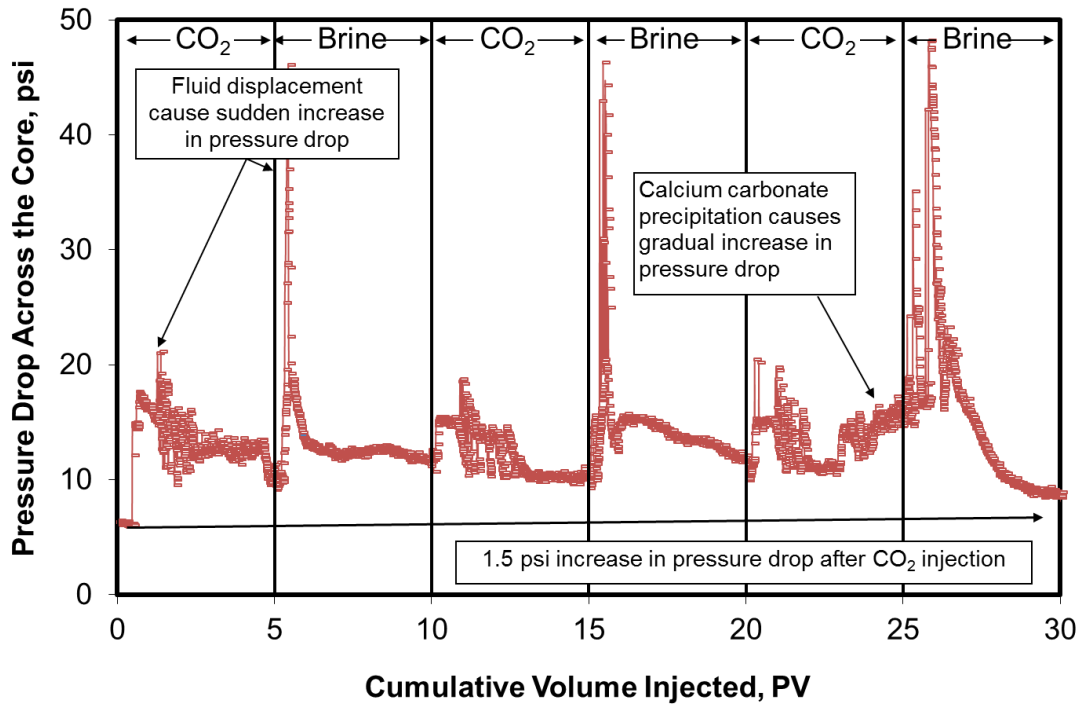
Fig. 4.1—Pressure drop across core #1 during CO 2 WAG injection (Reference case).
