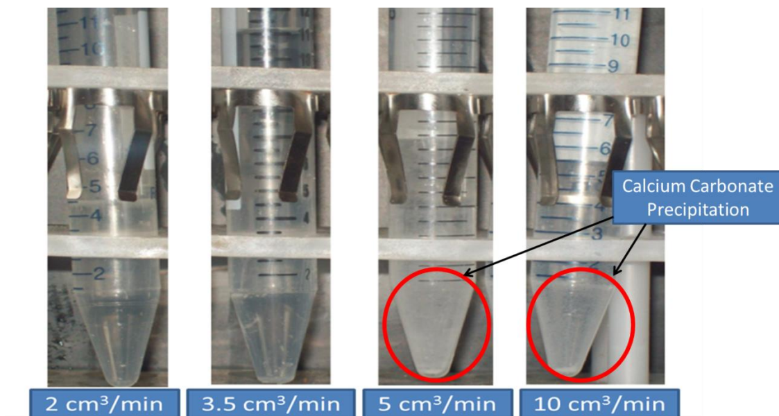
Fig. 4.12—Calcium carbonate was noted in the effluent samples just after alternating from CO 2 to brine at high flow rates.
