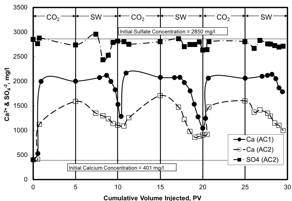
Fig. 8.5—Calcium concentration in the core effluent samples for core AC1 (WAG with seawater without sulfate injected), and calcium and sulfate concentrations for core AC2 (WAG with seawater injected).
