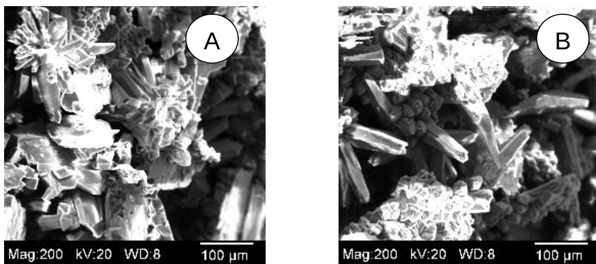
Fig. 8.6—SEM photomicrograph of calcium carbonate ( \text{CaCO}_3 ) particles noted in the core effluent samples for cores, A) AC1, and B) AC2.
