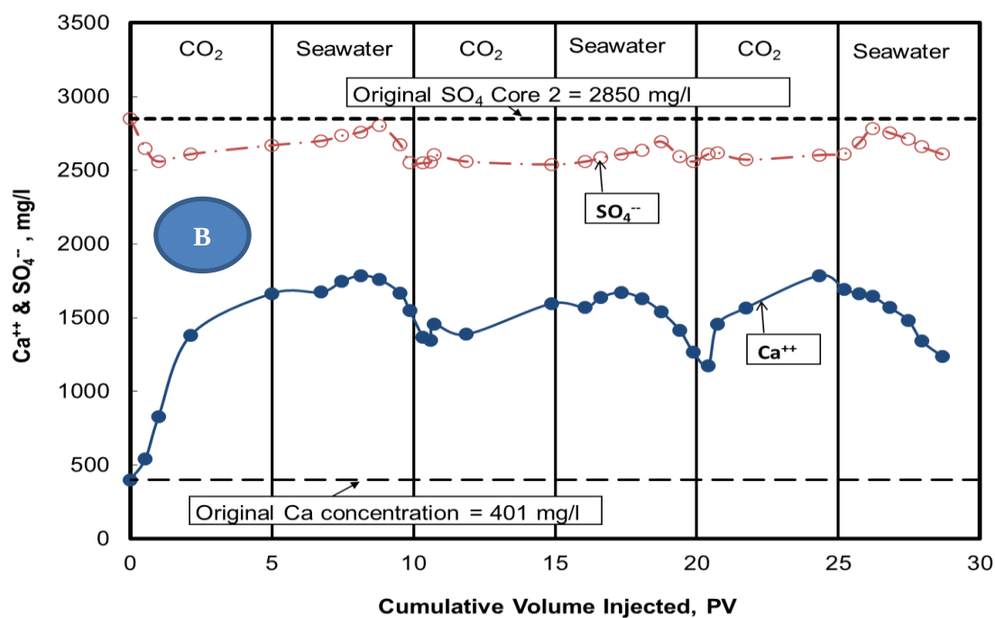
Fig. 5.1—Calcium and sulfate concentrations in the core effluent samples at a rate of 2 \text{ cm}^3/\text{min} , and 200^\circ\text{F} .
