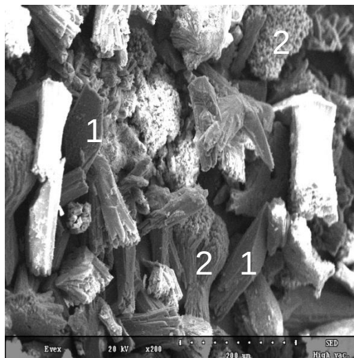
Fig. 8.16—SEM photo micrograph of the precipitated particles in the core effluent samples, SD1. XRD showed that the precipitated particles are; 1)Magnesian Calcite ( \text{Mg}_{0.13}\text{Ca}_{0.87}\text{CO}_3 ), 2) Aragonite ( \text{CaCO}_3 ).
