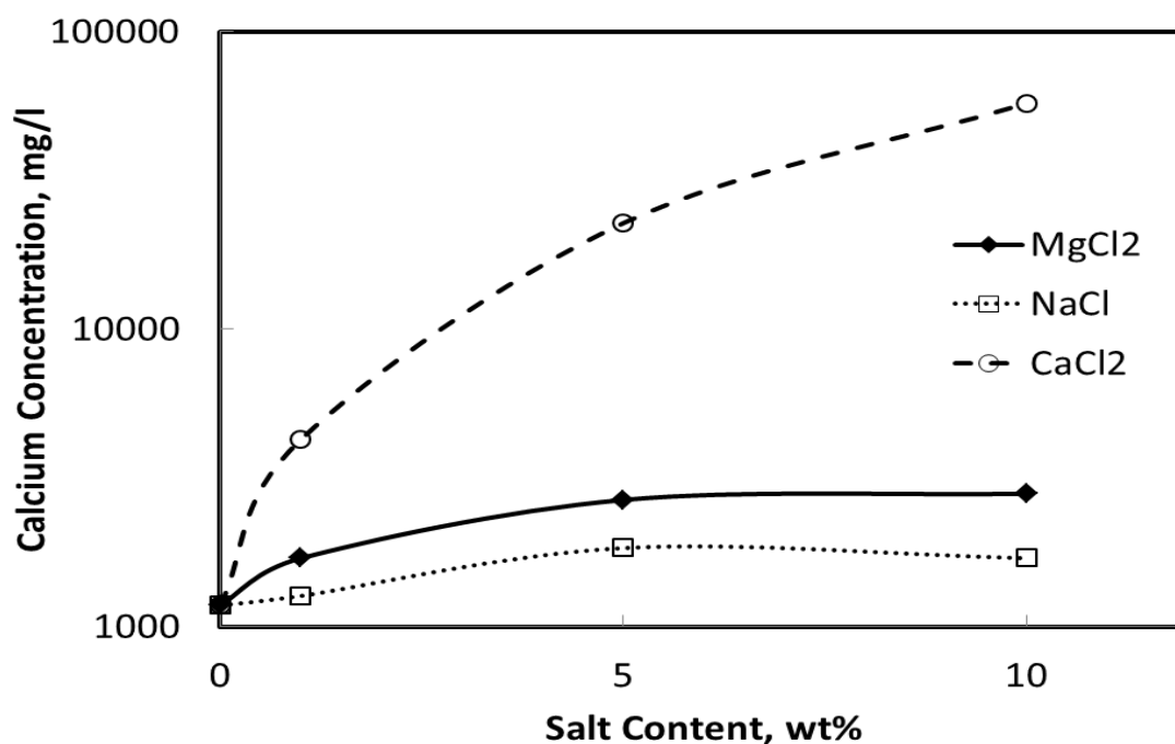
Fig. 5.6—Calcium concentration in the core effluent samples.
