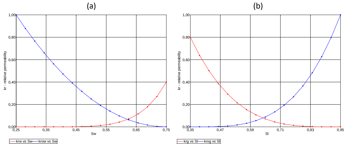
Figure 7. Relative permeability curves for water (a) and liquid (b).
