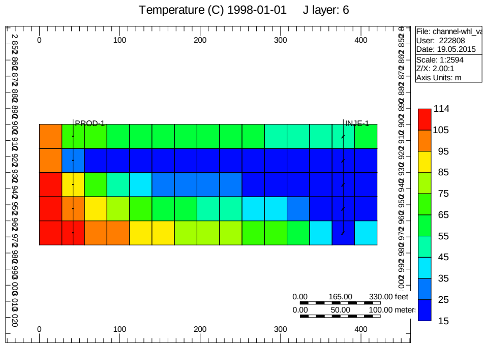
Figure 22. Temperature distribution for the channel model.
