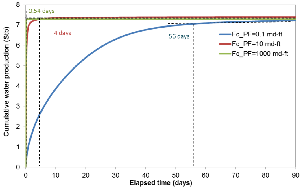
Figure 15. Cumulative water production comparison: Scenario 1, h = 90 ft, k_r\text{-}PF = 1
