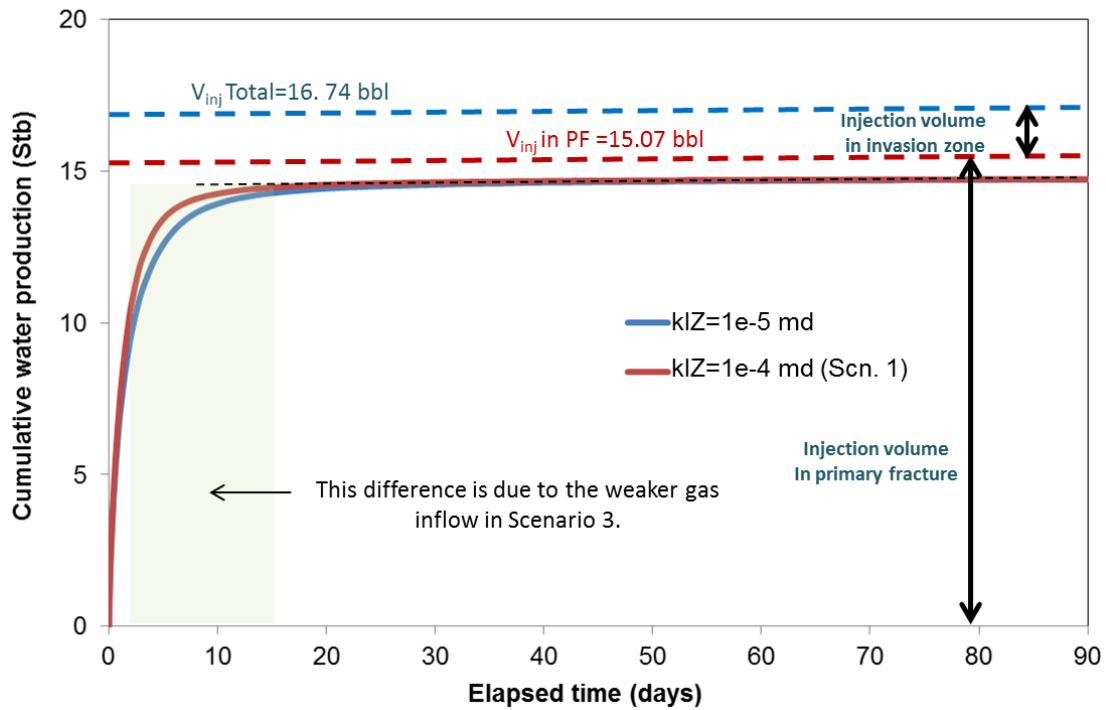
Figure 31. Cumulative water production comparison: Scenario 1 vs. Scenario 3, h = 180 ft, F_c\text{-PF} = 1 md-ft, k_r\text{-PF}1 , k_{IZ}=1e-5 md, k_r\text{-IZ}5 , p_c\text{-IZ}1
