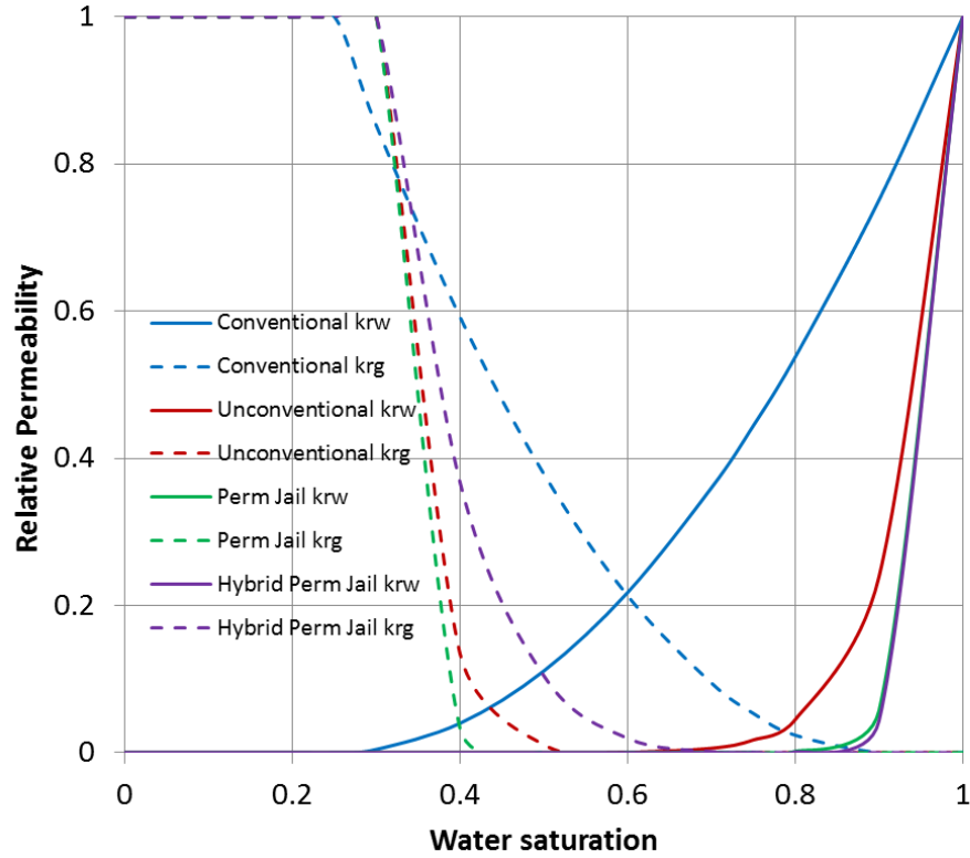
Figure 4. Four types of relative permeability profiles for secondary fracture system (Adopted from Alkouh and Wattenbarger 2013)
