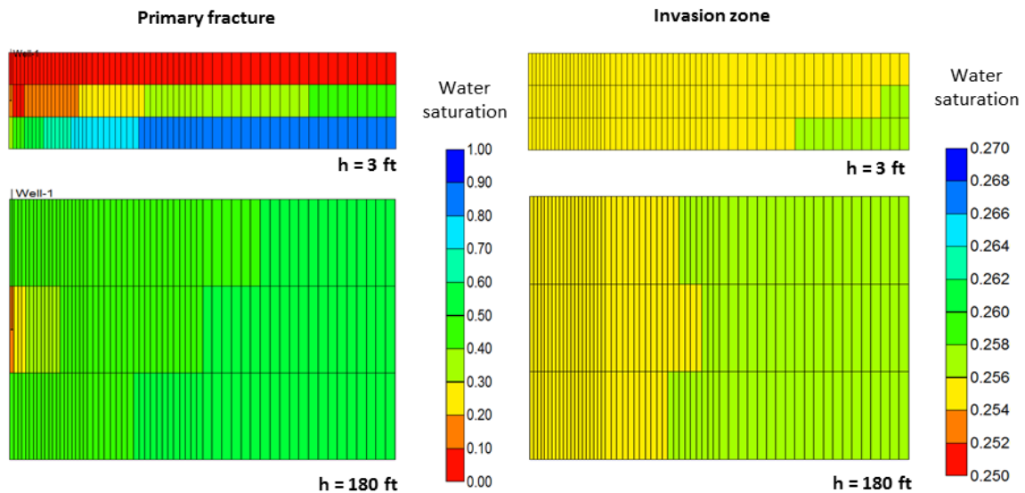
Figure 36. Water saturation distribution comparison after 1 day flowing: Scenario 3, k_{IZ} = 1e-5 md, k_f -IZ-1, p_c -IZ-5, h = 3 ft vs. h = 180 ft
