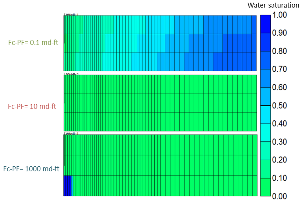
Figure 16. Primary fracture water saturation profile comparison at 10 days: Scenario 1, h = 90 ft, k_{r-PF} = 1
