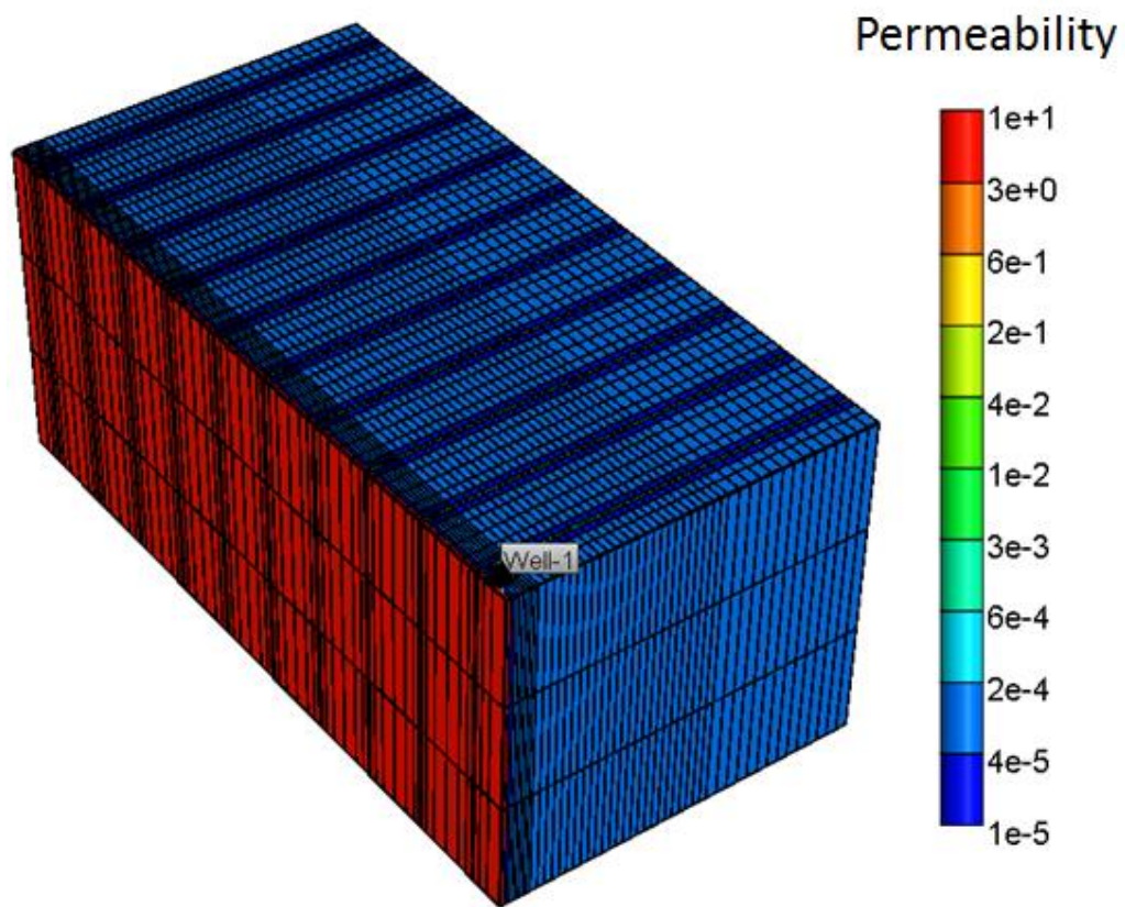
Figure 42. 3D numerical simulation model of Scenario 4
