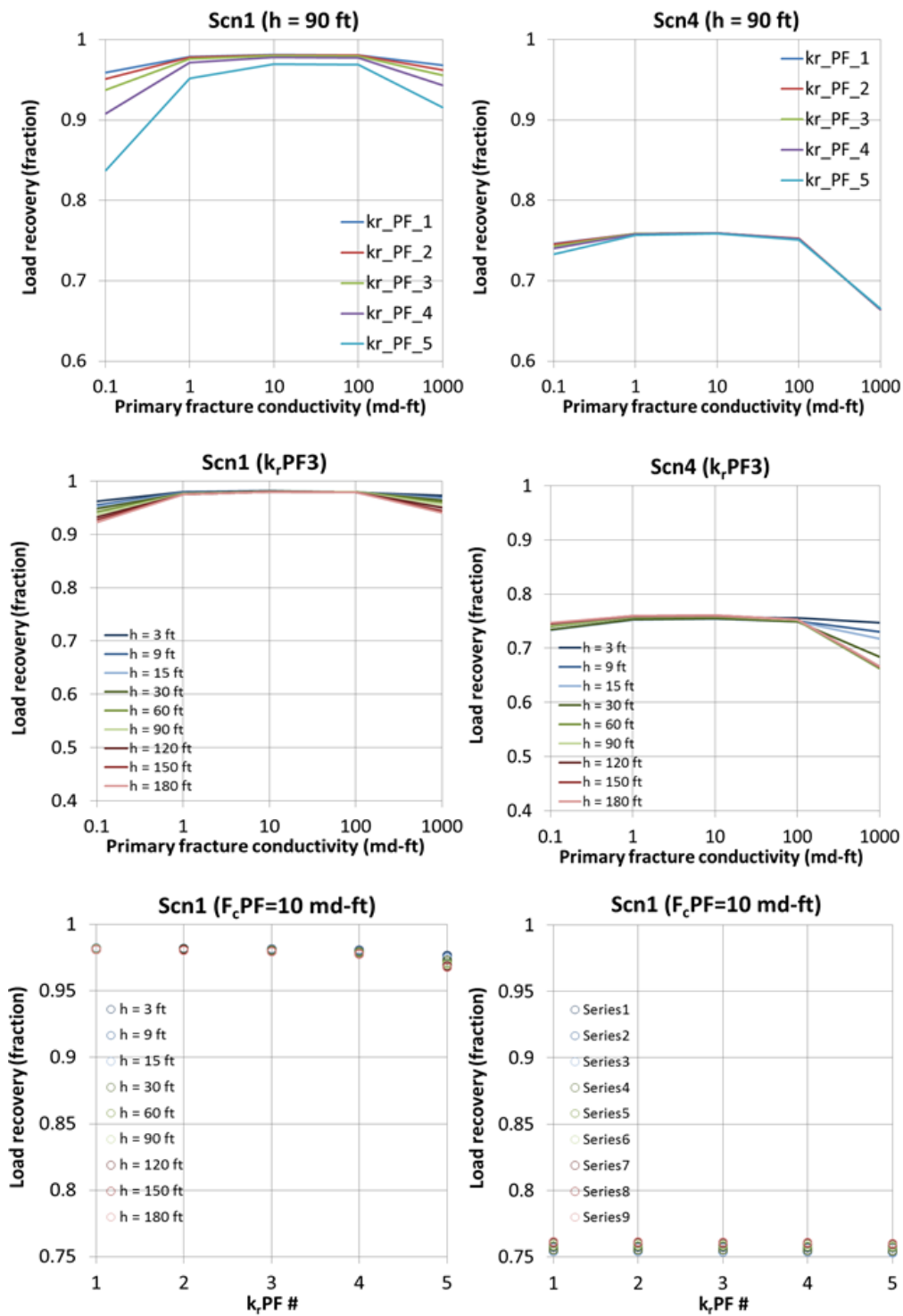
Figure 43. Primary fracture's impacts on load recovery comparison between Scenario 1 and Scenario 4
