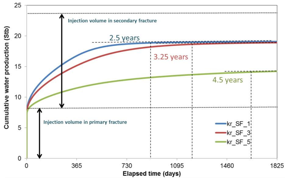
Figure 23. Cumulative water production comparison: Scenario 2, h = 90 ft, F_c\text{-SF} = 0.001 md-ft
