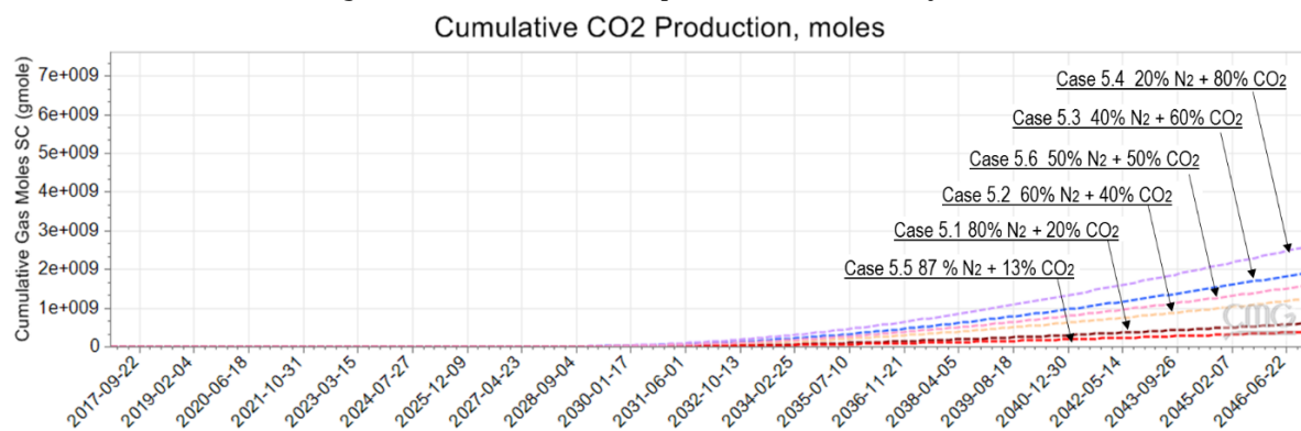
Figure 47 – Cumulative CO 2 injection. Mixture Injection
