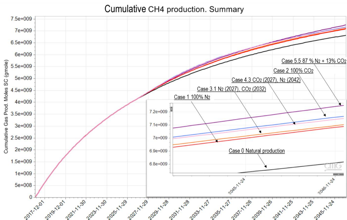
Figure 52 – Cumulative CH 4 production, summary
