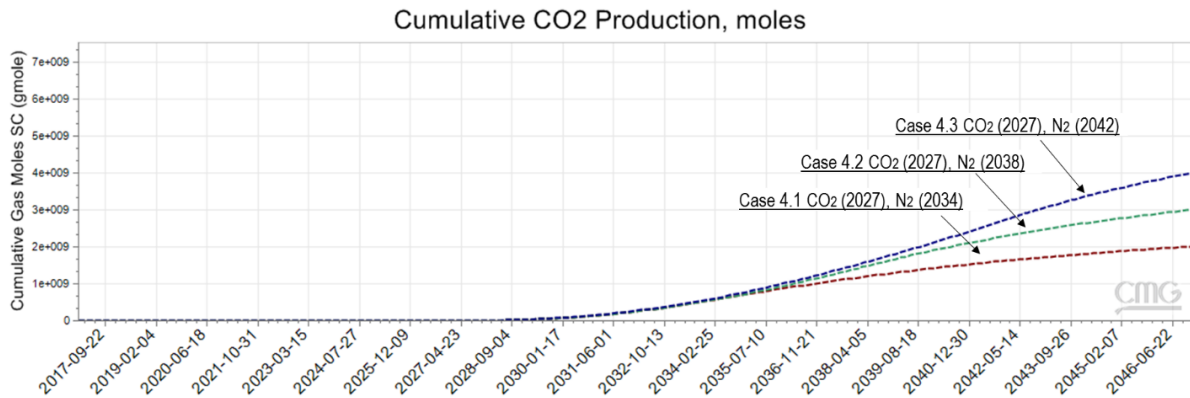
Figure 43 – Cumulative CO 2 production. CO 2 - N 2 alternating injection
