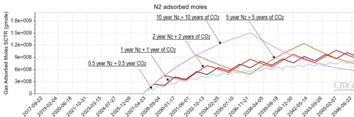
Figure 57 – N 2 adsorbed moles. Case 3b
