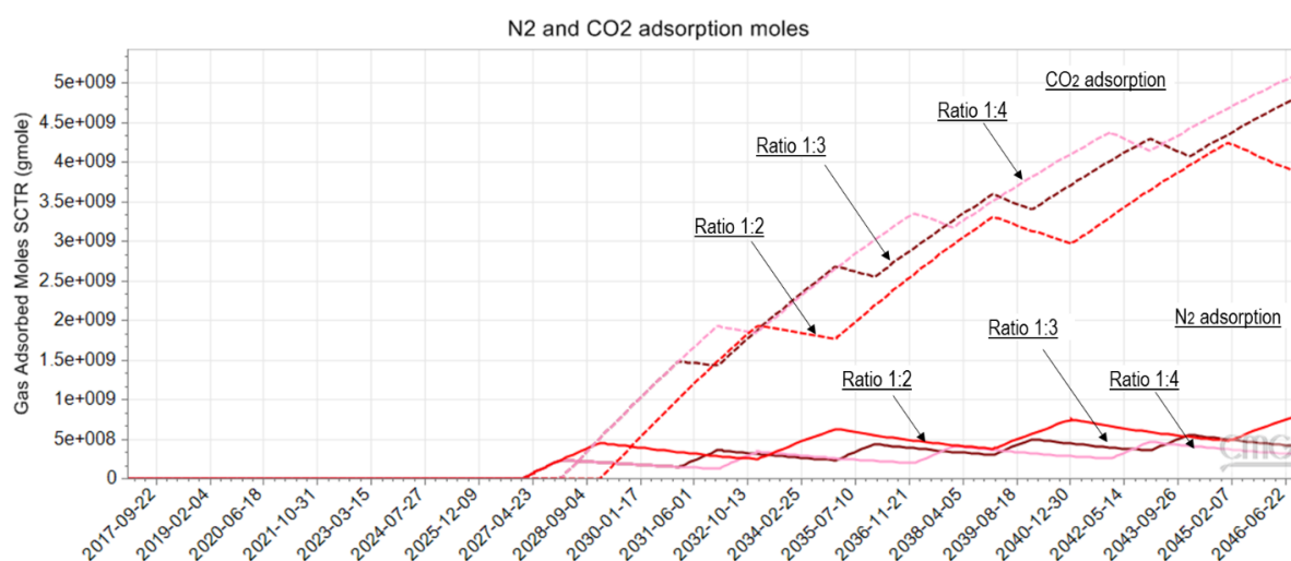
Figure 59 – CO 2 and N 2 adsorption. case 3c
