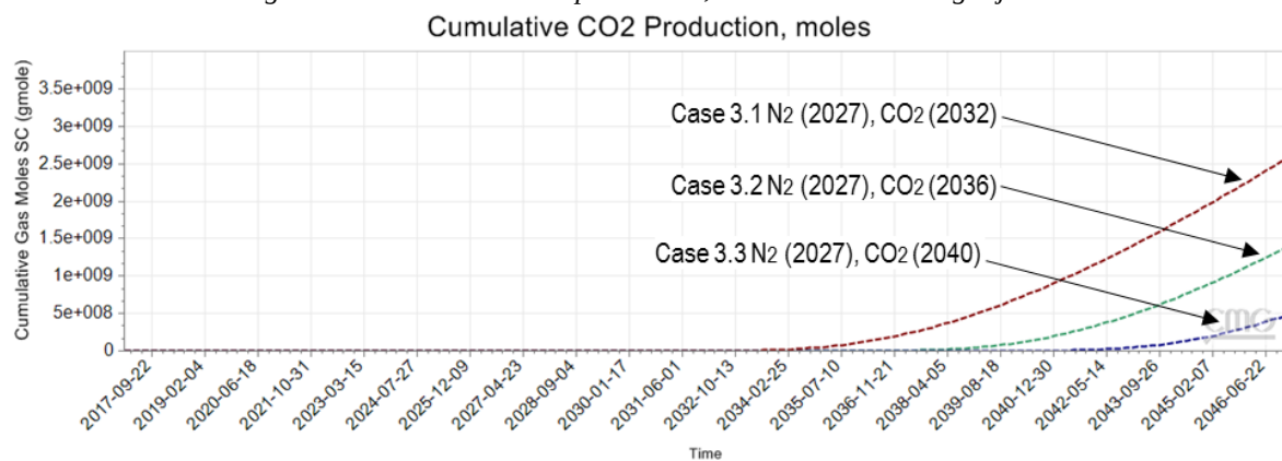
Figure 38 – CO 2 cumulative production, N 2 -CO 2 alternating injection
