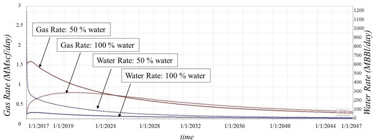
Figure 28 – Gas and water rate curves for cases with 100% and 50% of initial water in place
