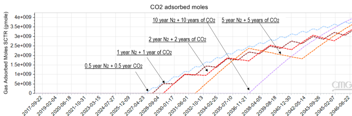
Figure 58 – CO 2 adsorbed moles. Case 3b
