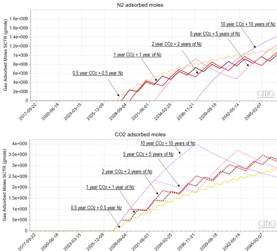
Figure 62 – Case 4b. N 2 and CO 2 adsorption characteristics.
