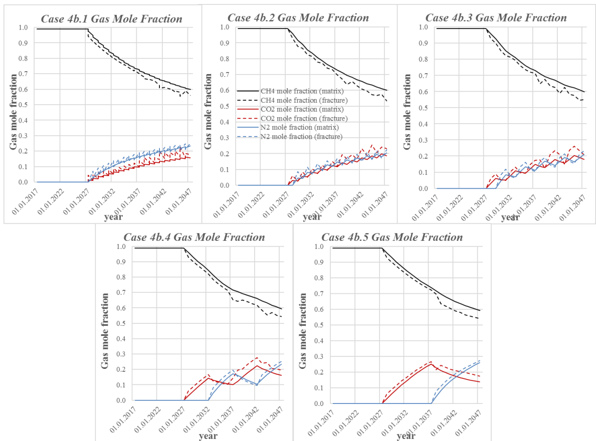
Gas mole fraction. Case 4b
