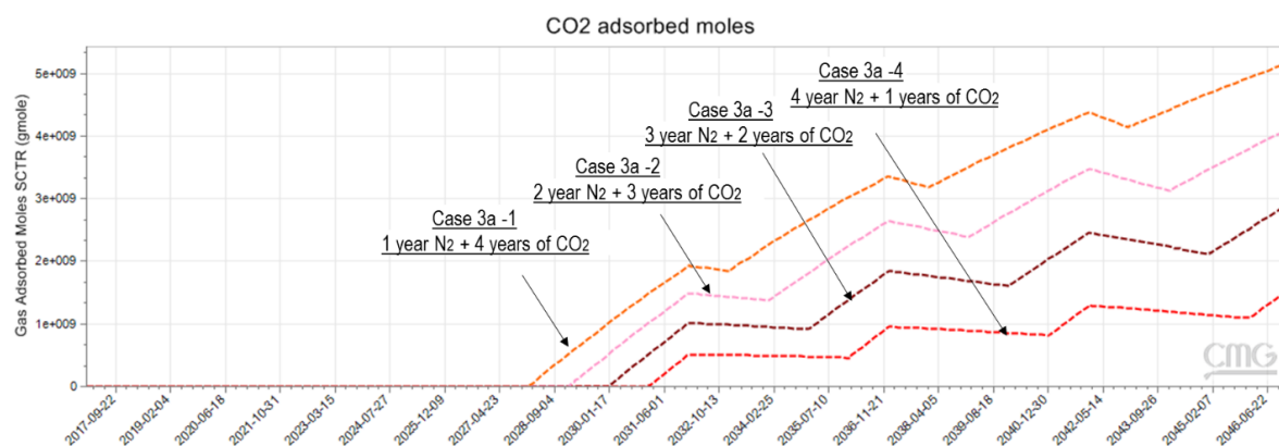
Figure 56 – CO 2 adsorption characteristics, case 3a
