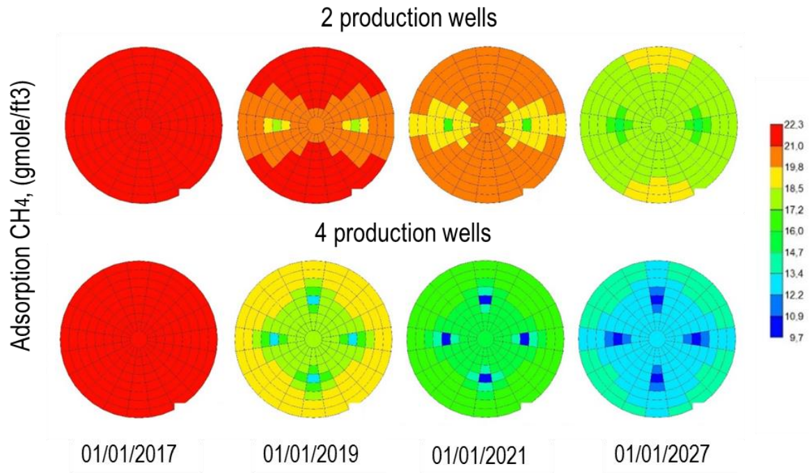
Figure 54 – CH_4 adsorption. Row 1 – Case 5.5, Row 2 – Case 6
