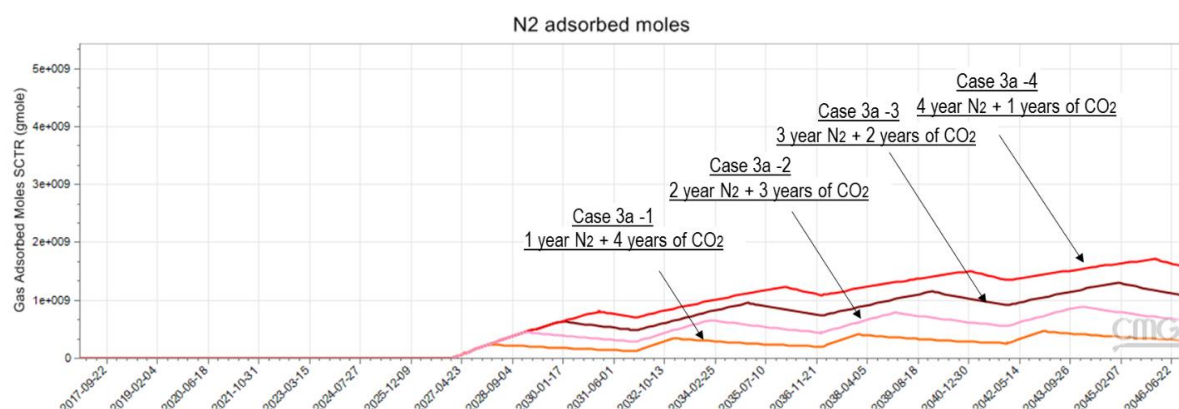
Figure 55 – N 2 adsorption characteristics, case 3a
