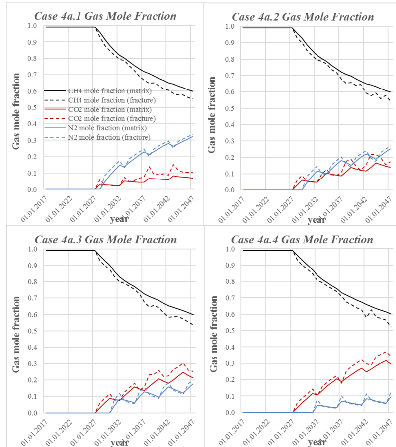
Gas mole fraction. Case 4a
