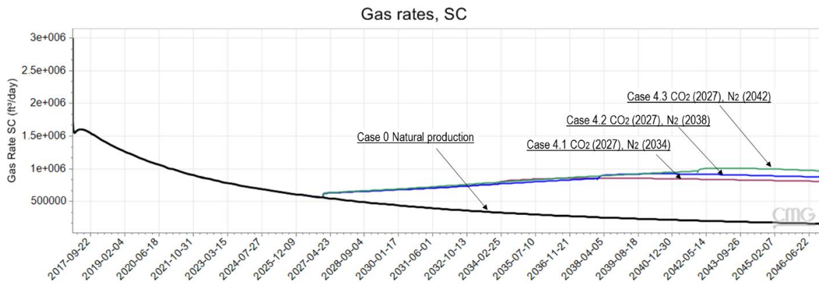
Figure 44 – Gas rates. CO 2 - N 2 alternating injection
