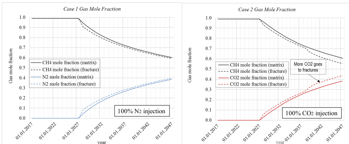
Figure 32 – Gas mole fraction, case 1 and case 2
