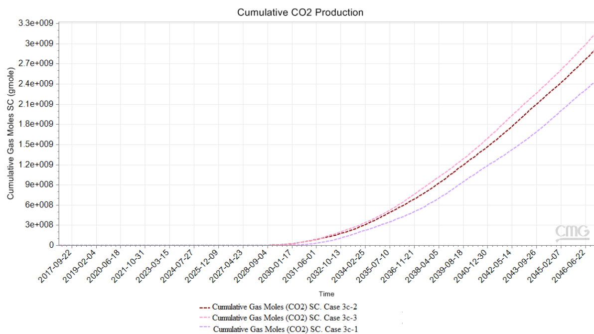
Case 3b. CO 2 and N 2 cumulative production
