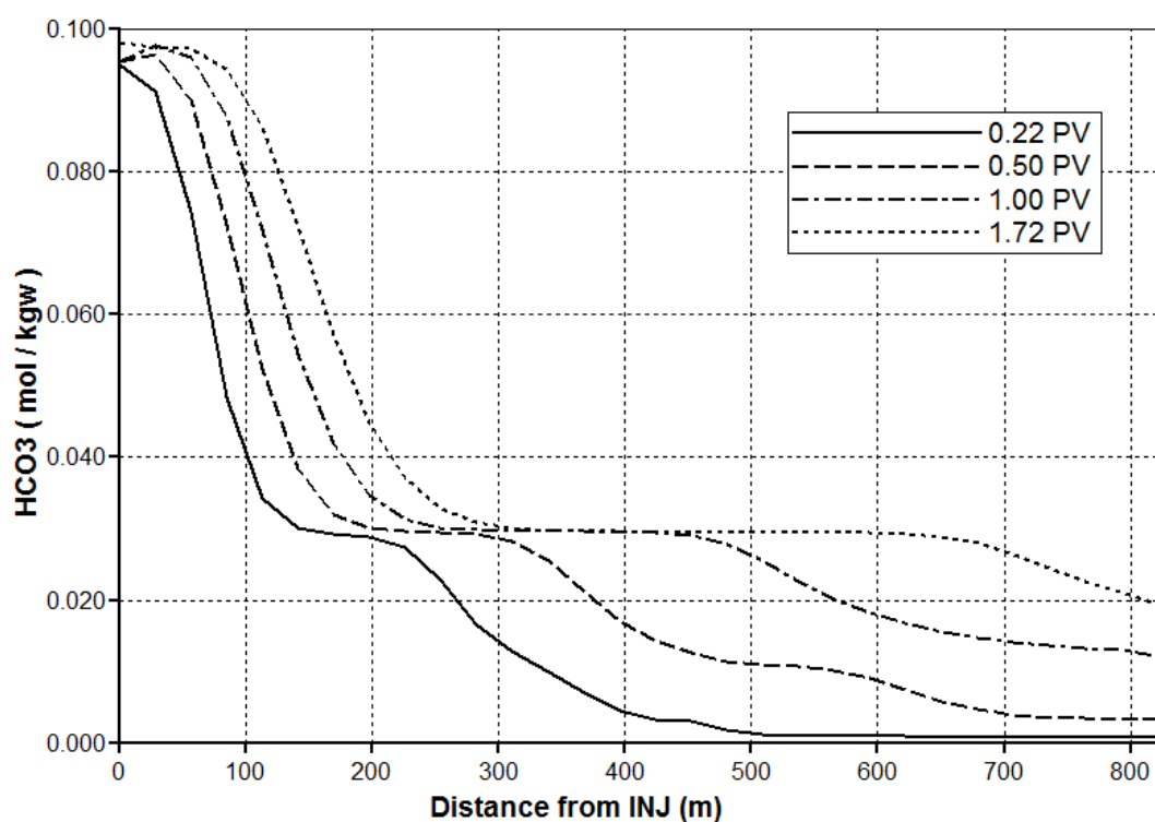
Figure 6.19. HCO 3 concentration profile for L2 at different times (measured in pore volumes).
