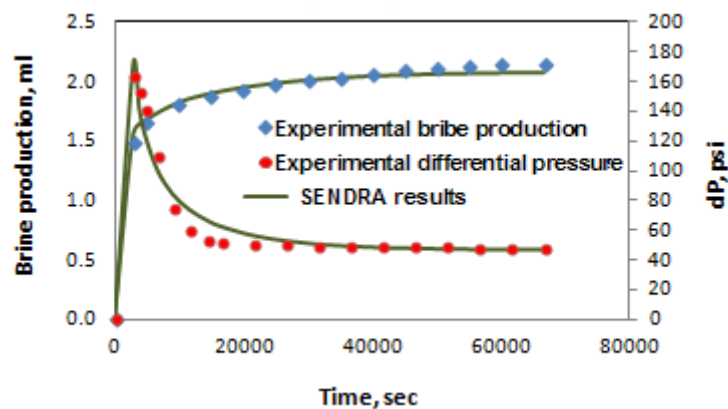
Figure 11: Brine production and pressure differential in the core flooding experiment
