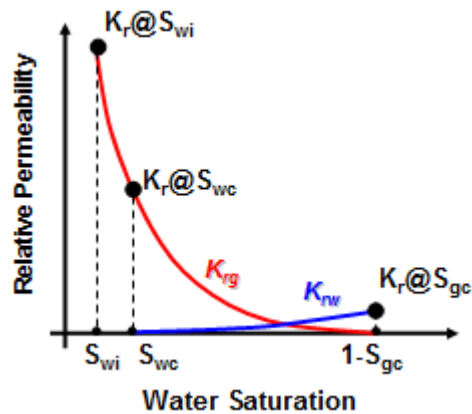
Figure 3: Reduced effective permeability due to phase trapping damage (Bennion et al, 2006)
