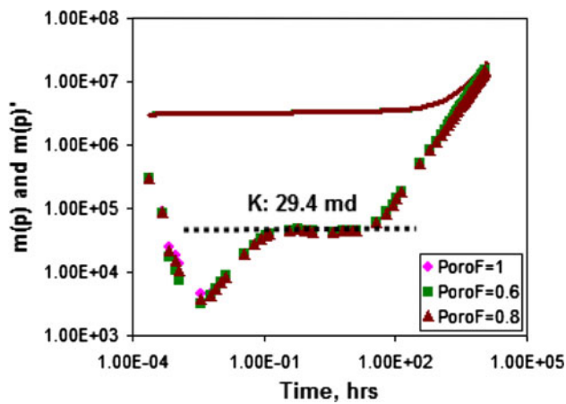
Fig. 11 Effect of fracture porosity ( \text{Porof} ) on welltest permeability
