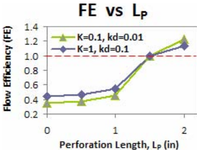
Figure 12. Simulation results related to the effect of perforation tunnels length on flow efficiency of a damaged core.
