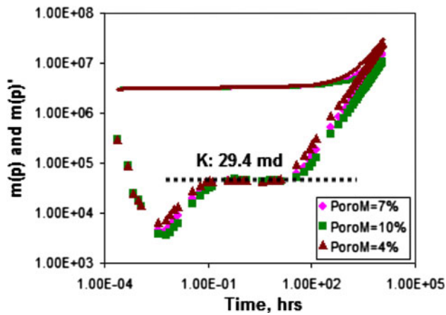
Fig. 10 Effect of matrix porosity ( \text{Porom} ) on welltest permeability
