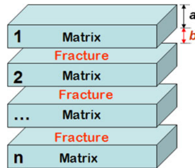
Fig. 3 Kazemi model parameters for naturally fractured reservoirs
