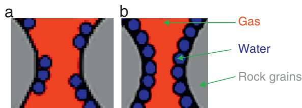
Fig. 1. The concept of normal and sub-normal initial water saturation. a: Sub-normal initial water saturation ( S_{wi} < S_{wc} ). b: Normal initial water saturation ( S_{wi} = S_{wc} ).
