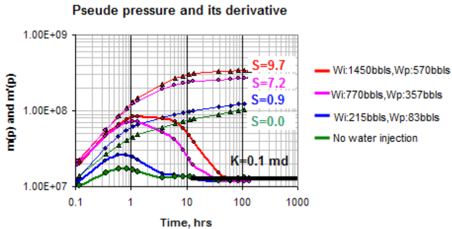
Figure 17: Effect of phase trap damage on skin factor
