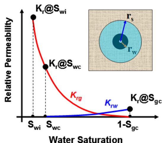
Fig. 2. Typical gas and water relative permeability curves, indicating how near wellbore permeability is reduced due to water invasion.
