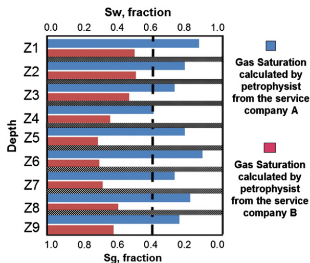
Fig. 3. Water saturation variations along wellbore in the tight sand formation in Perth Basin (total net thickness of the porous sand intervals: 370 ft).
