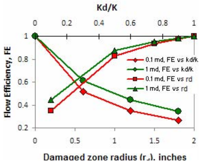
Figure 8. Effect of damaged zone permeability and radius on flow efficiency.
