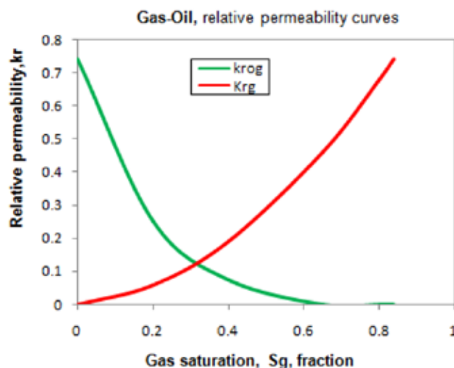
Figure 4b. Capillary pressure and relative permeability for a gas-oil system.
