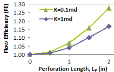
Figure 27: Effect of perforation tunnel length on flow efficiency
