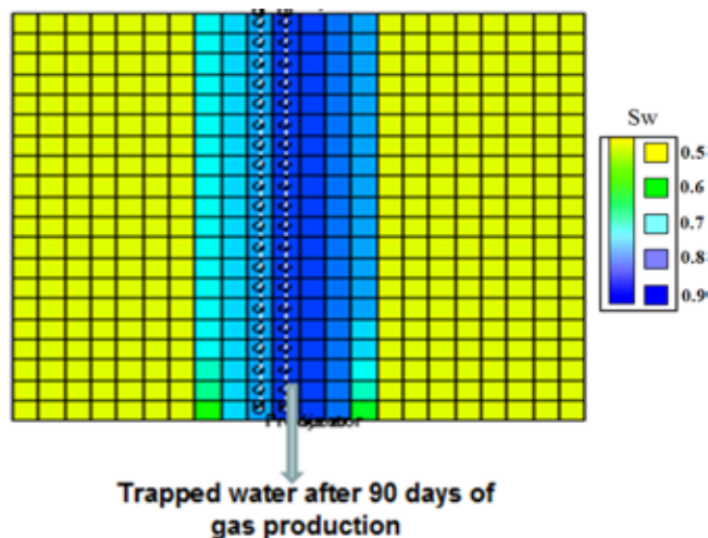
Figure 6b. Water saturation distribution at the end of the gas production and clean-up period (water damage).
