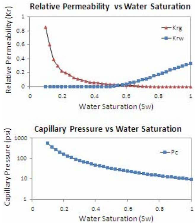
Figure 1. Typical relative permeability and capillary pressure curves for a tight sand formation.
