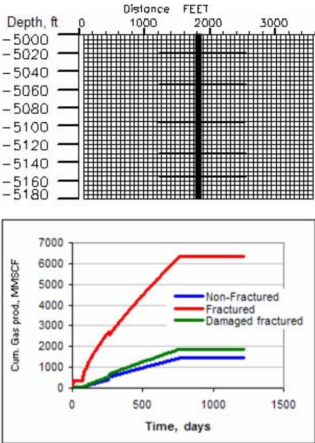
Figure 18. Simulation results related to the effect of mechanical damage to natural fractures on gas recovery.
