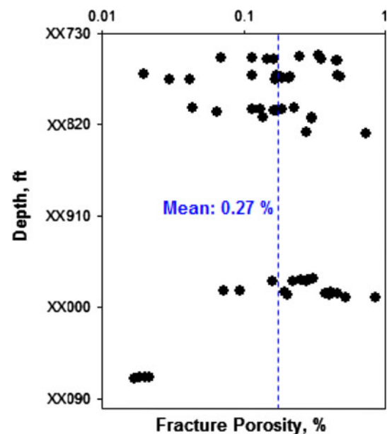
Fig. 17 Fracture porosity data from Image Log processing results
