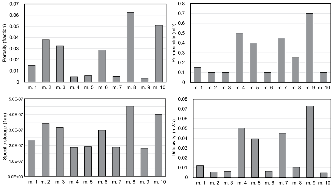
Figure 3. Calculated crystalline basement porosity, permeability, specific storage and diffusivity for 10 different models.
