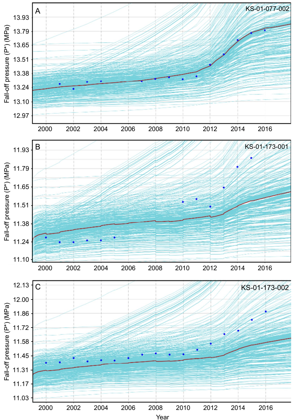
Figure 2. Matching the measured Arbuckle pressures for wells (a) “KS-01-077-002,” (b) “KS-01-173-001,” and (c) “KS-01-173-002” (matched model 3; Table S14). Blue points are the historical pressure data, light blue curves show different simulation runs, and the red curve shows the best model determined by tuning the basement properties (permeability and porosity). More than 2,000 runs are performed to obtain the best match.
