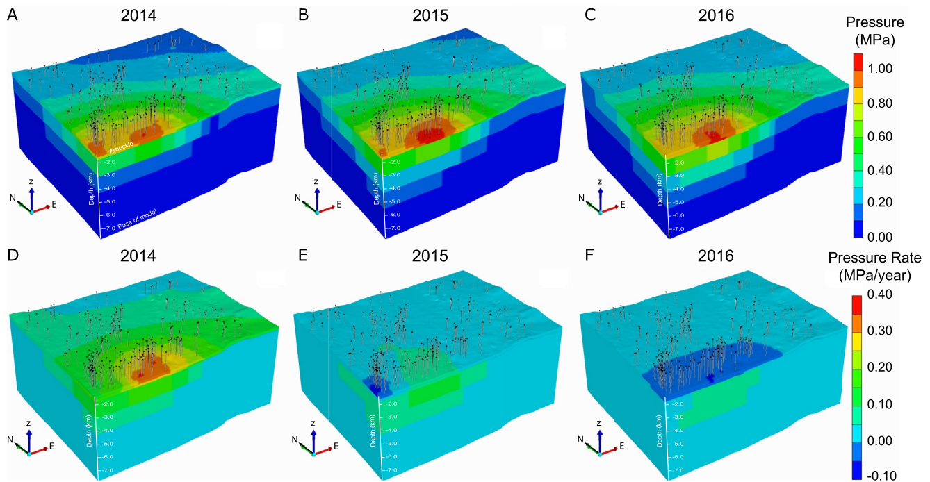
Figure 4. (a–c) Cumulative pressure change (MPa) and (d–f) annual pressure change rate (MPa/year) across the south-central Kansas model area (Figure 1) since 2000, obtained from geological and numerical history matching. Vertical exaggeration is 10X.
