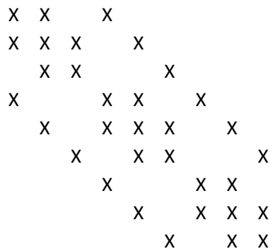
Figure 2.5 Jacobian structure of a single equation system with single variable and discretized in a 5-grid system
