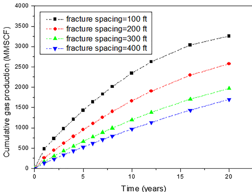
Fig 9. Effect of fracture spacing on the cumulative gas production of shale gas reservoirs.
