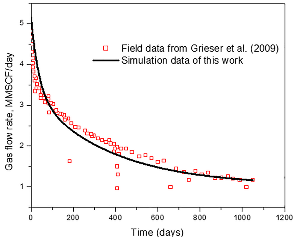
Fig 3. Comparison between simulation results and the field data of Barnett shale.
