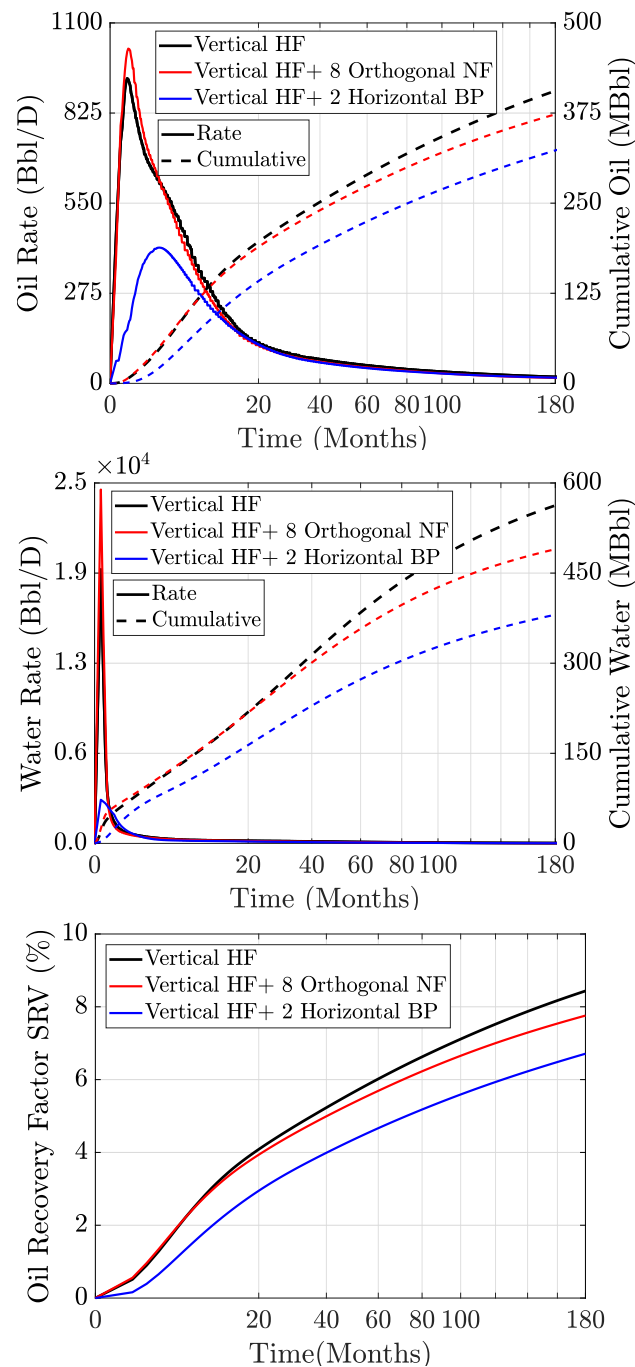
Figure 11. Simulation case 2: 15 years of reservoir fluid production obtained by varying hydraulic fracture geometry. Fracture scenario #1 is the reference case, which only has three vertical hydraulic fractures (HF) (black line). Fracture scenario #2 has three vertical hydraulic fractures and eight orthogonal natural fractures (NF) (red line). Fracture scenario #3 has three vertical hydraulic fractures and two horizontal bedding planes (BP) (blue line). The fracture scenarios #1 and #2 have a vertical hydraulic fracture permeability of 2000 mD. Fracture scenario #3 has a vertical hydraulic fracture permeability reduced by 90% (200 mD).
