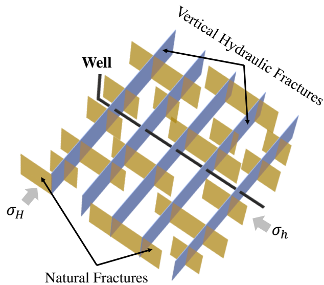
Figure 7. Schematic figure of an orthogonal fracture network. Adapted from: [78].
