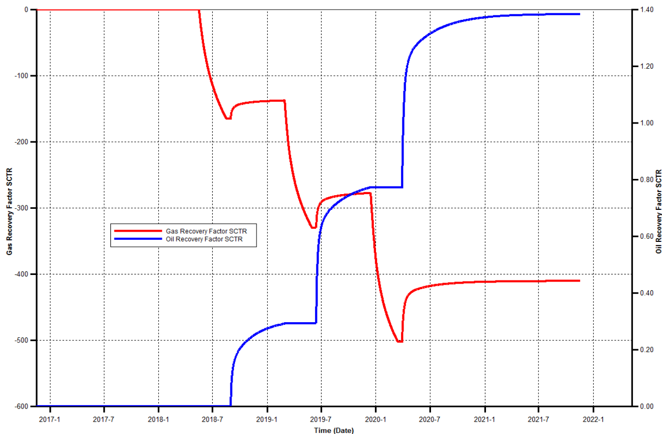
Fig. 18 Oil recovery factor and CO 2 recovery factor during CO 2 solubility process
