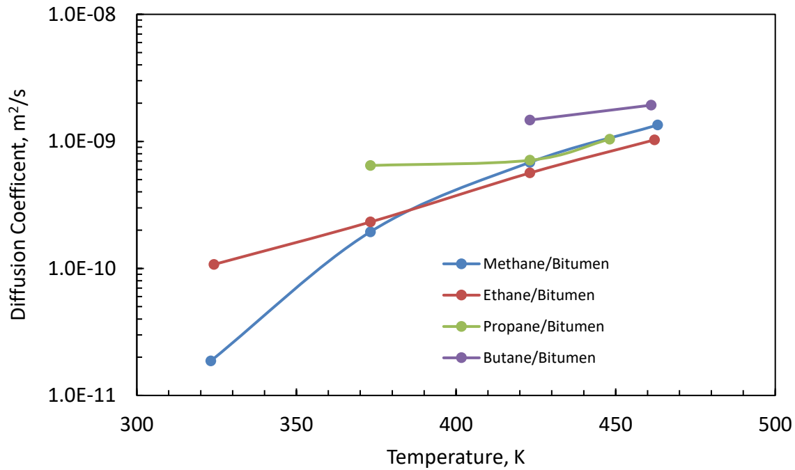
Figure 3.5: Estimated diffusion coefficients for different solvents/bitumen mixtures at 20 bar.
