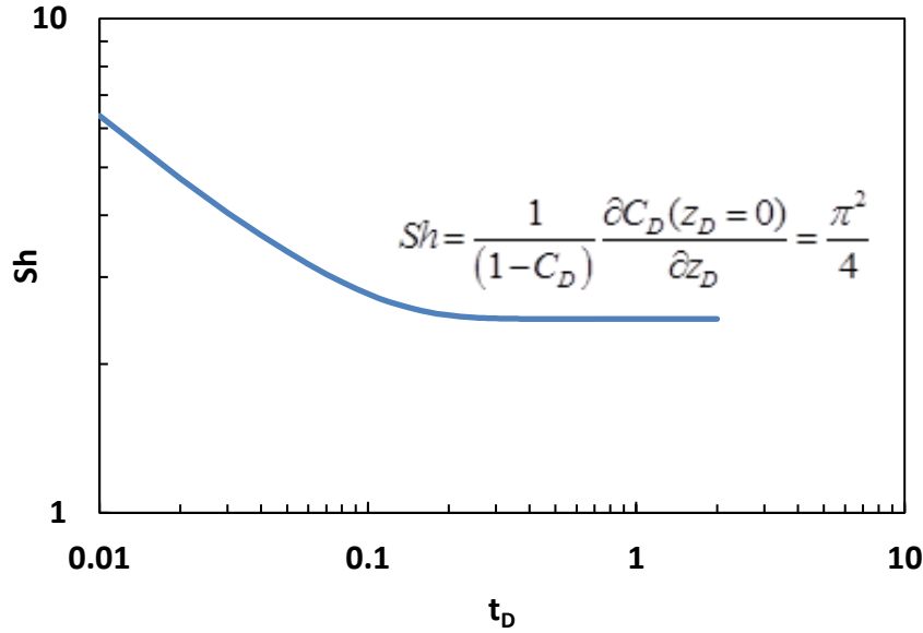
Figure 3.2: Sherwood number versus dimensionless time.
