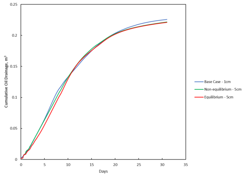
Figure 5.16: Cumulative oil drainage for Propane/Bitumen system at 2000 kPa and 75 °C – 5 cm grid block size.
