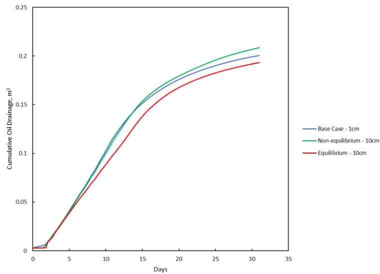
Figure 5.19: Cumulative oil drainage for Propane/Bitumen system at 1600 kPa and 75 °C – 10 cm grid block size.
