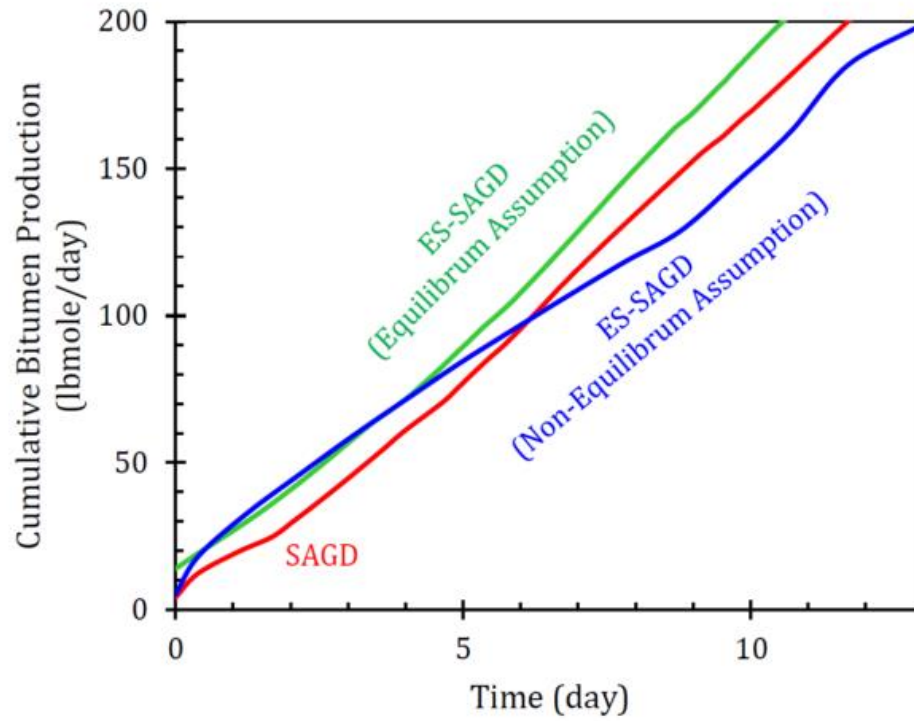
Figure 2.6: Oil production steam gravity drainage processes. Red, blue, and green lines are SAGD, ES-SAGD (non-equilibrium assumption), and ES-SAGD (equilibrium assumption) (Bayestehparvin et al. 2017).
