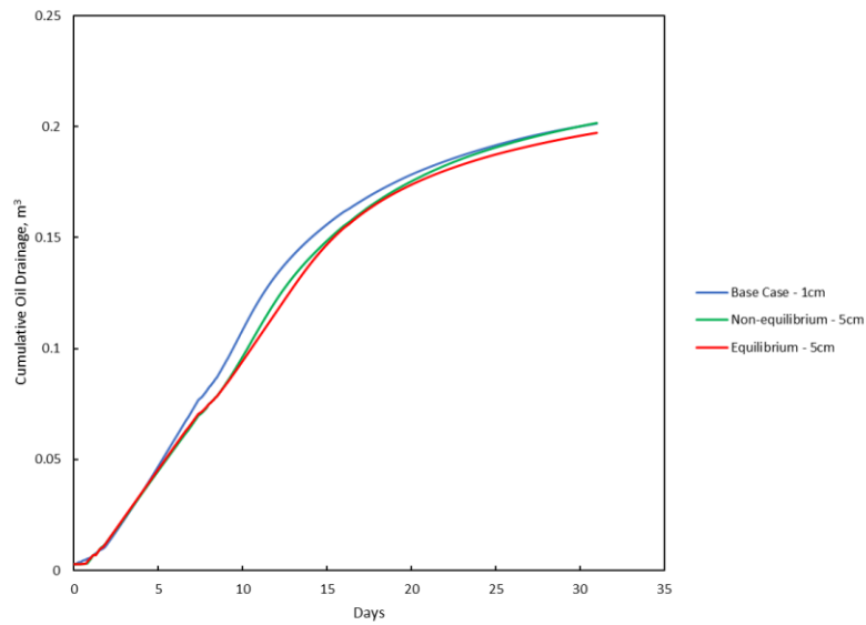
Figure 5.18: Cumulative oil drainage for Propane/Bitumen system at 1600 kPa and 75 °C - Equilibrium versus Non-equilibrium – 5 cm grid block size.
